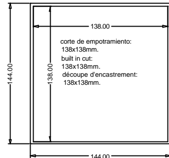
VISTA FRONTAL FRONT VIEW VUE DE FACE
