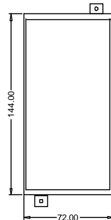
VISTA FRONTAL FRONT VIEW VUE DE FACE
