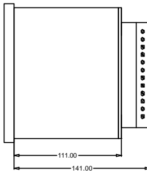
VISTA LATERAL SIDE VIEW VUE DE COTE
