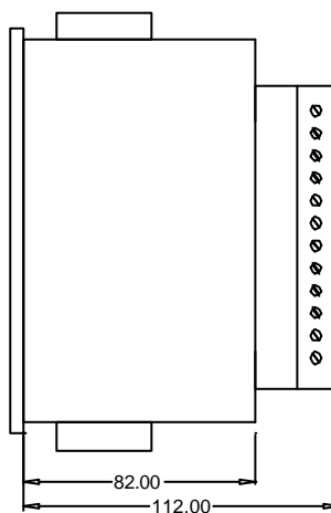
VISTA LATERAL SIDE VIEW VUE DE COTE
